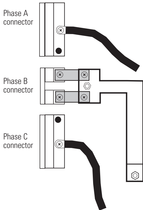
Phase connectors wired for three phase operation
