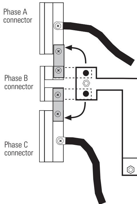
Phase connectors wired for single phase operation
